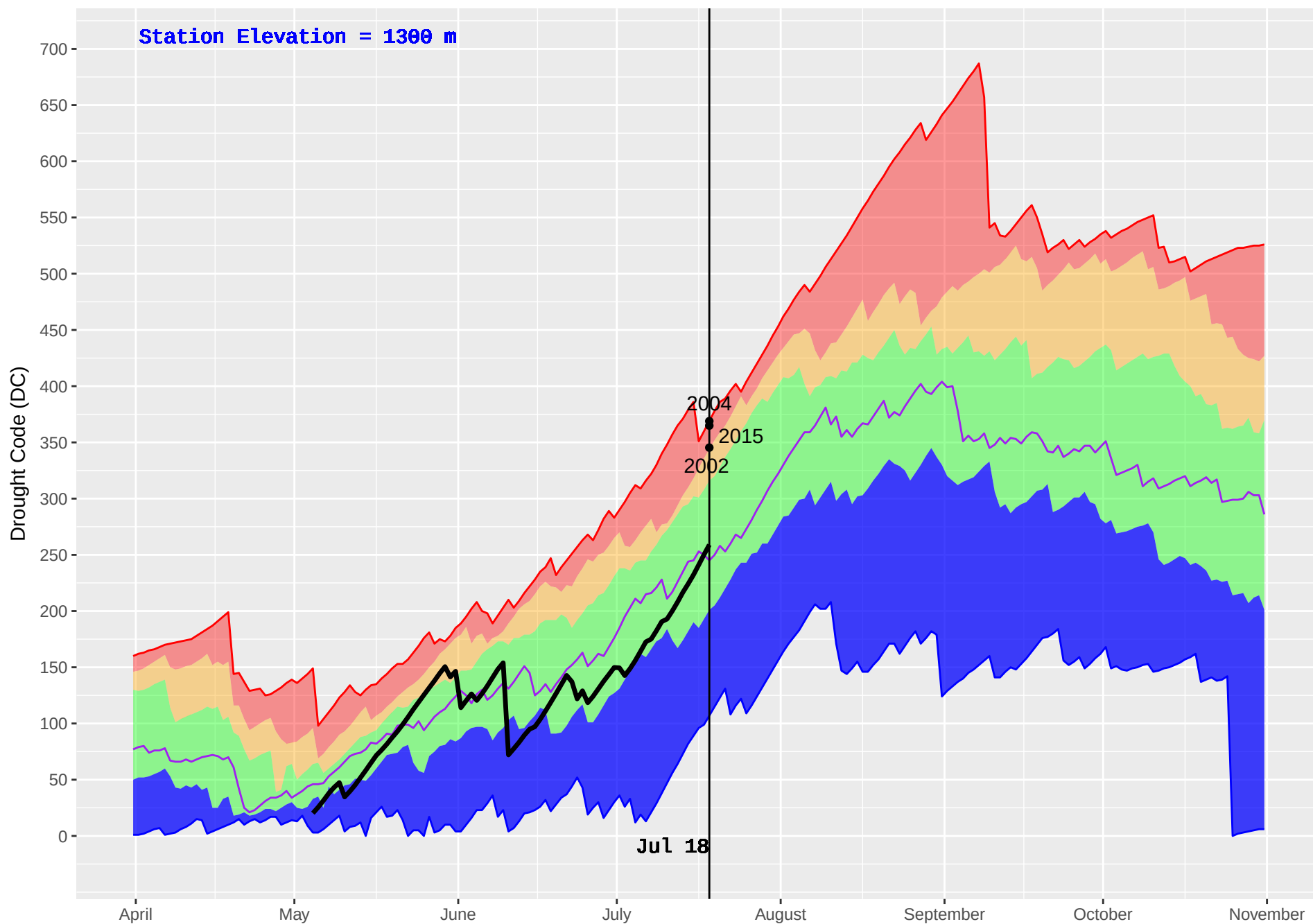
MARION (367) : Historical (1994–2016) and Current (2018) Daily Drought Code (DC)
